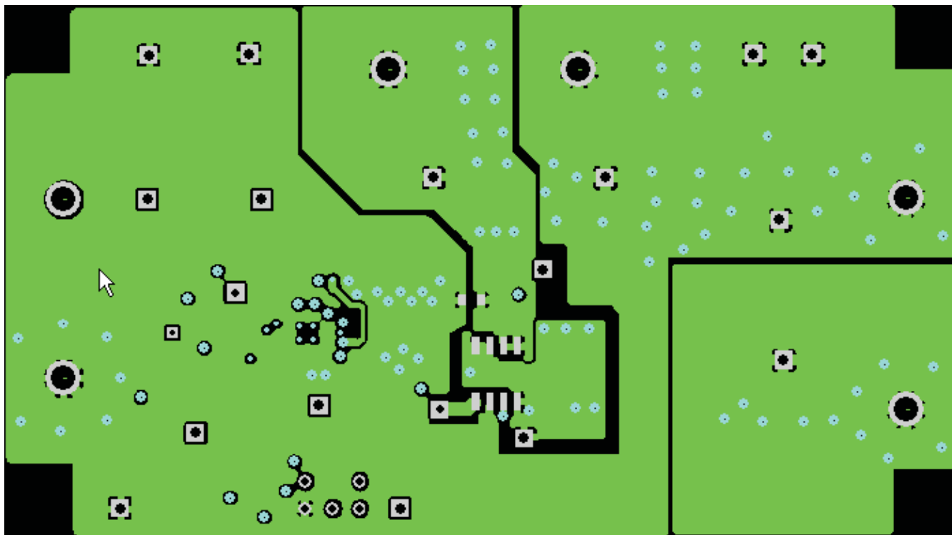
Figure 5. Bottom Layer Copper
